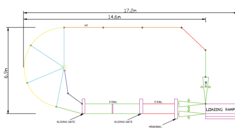
46 Head Plan with Curved Tub
